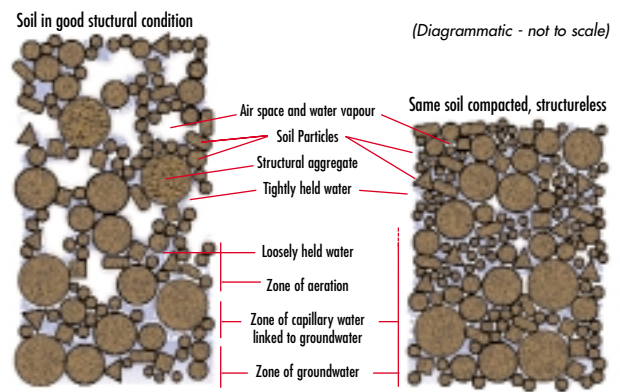
FIGURE 2: COMPACTION EFFECTS ON SOIL STRUCTURAL CONDITIONS
